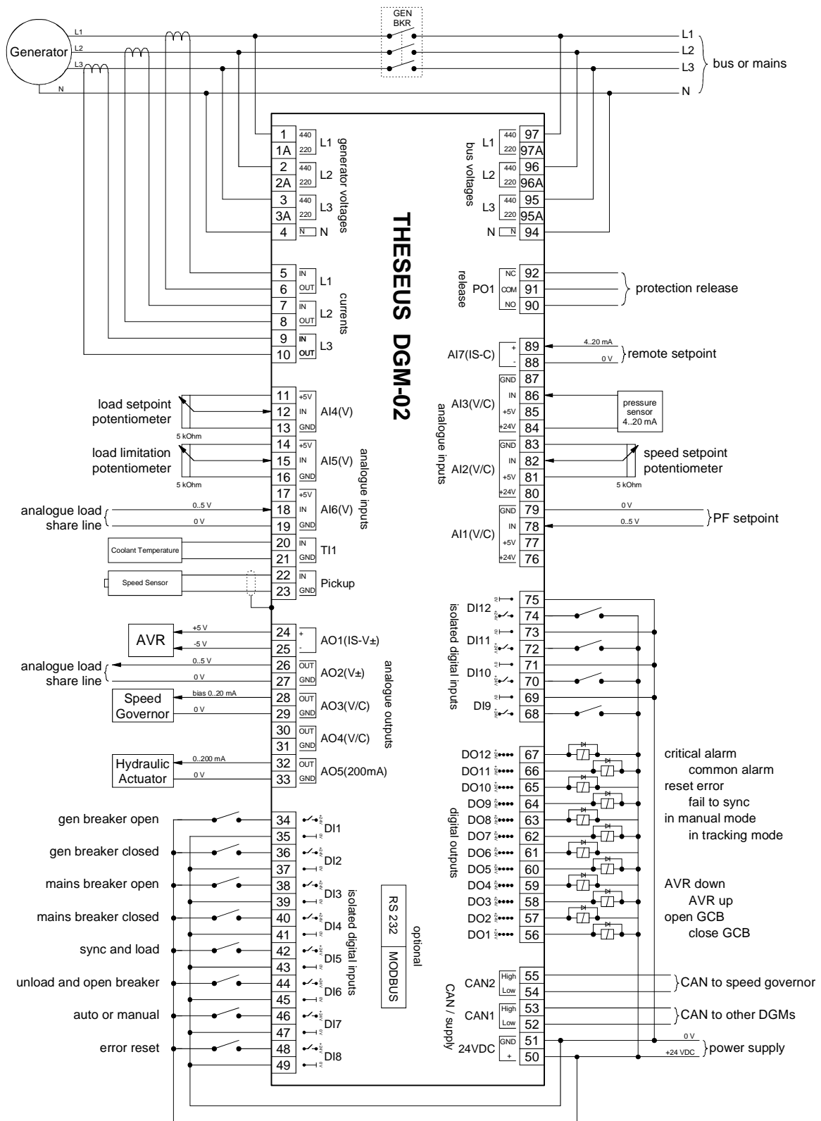
Figure 7: Exsample of wiring diagram
