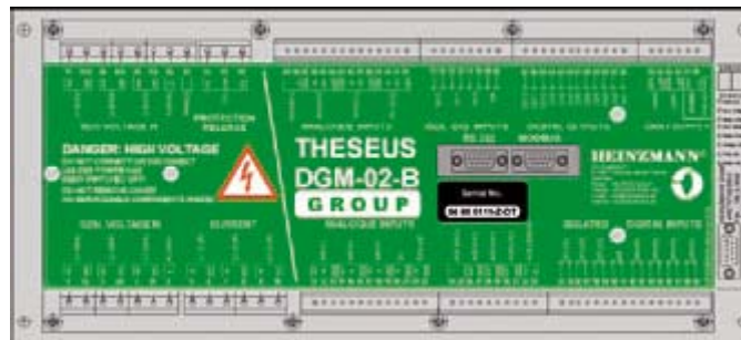
Figure 5: DGM-02 Group to Mains
