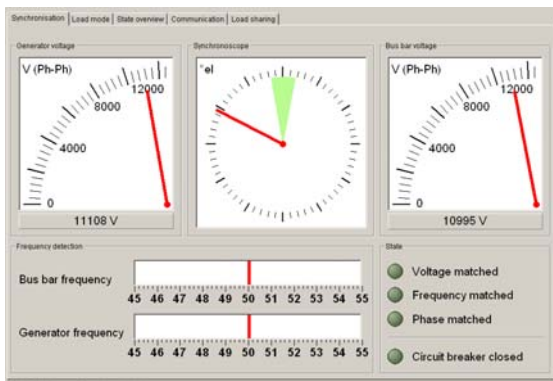
Figure 15: Window at synchronizing
