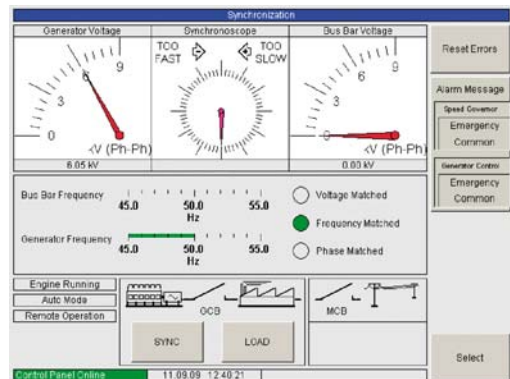
Figure 11: Screen for synchronizing
