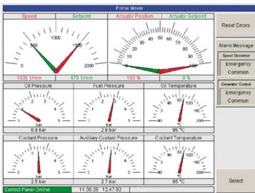
Figure 10: Screen for speed governor
