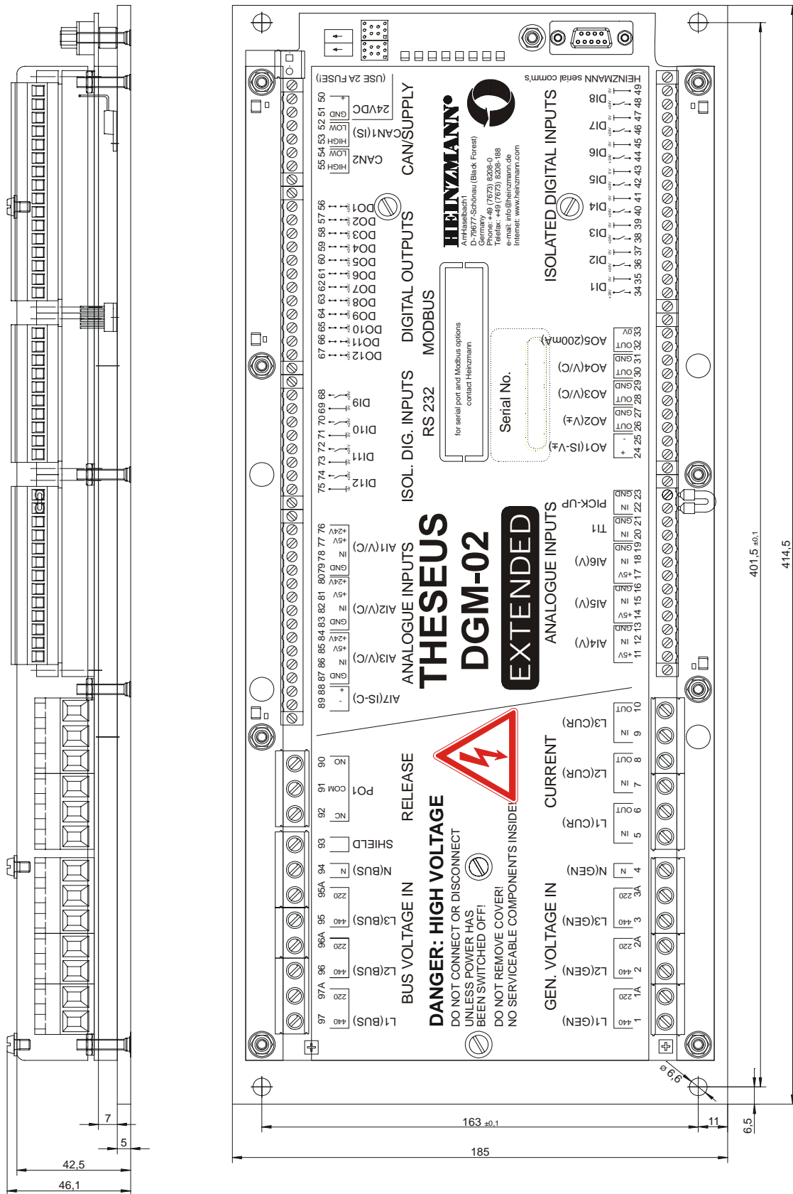
Figure 6: Dimensional drawing of DGM-02
