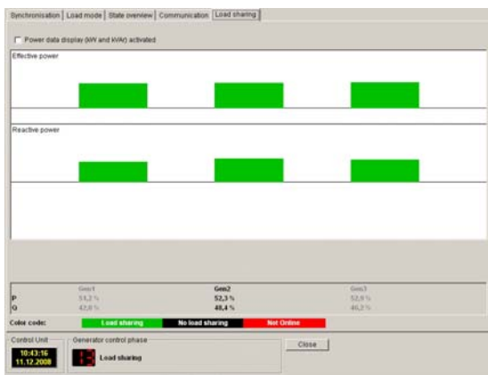
Figure 17: Window to monitor load sharing
