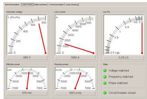
Figure 16: Window to measure generator load
